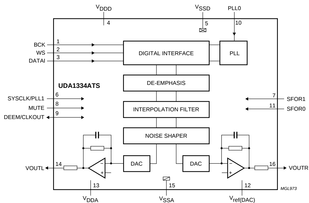
Fig.1 Block diagram.
